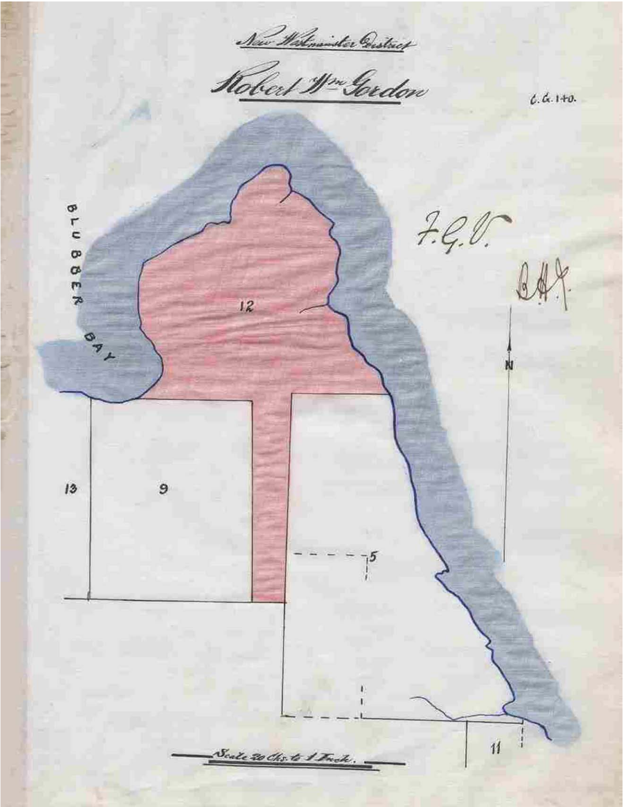
1888 Robert William Gordon District Lot 12 Survey
